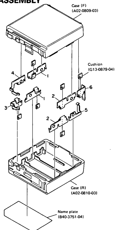
BT-6 DISASSEMBLY
