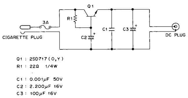
PG-3F CIRCUIT DIAGRAM
