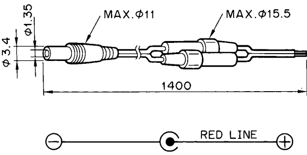
PG-2W MAIN EXTERNAL DIMENSIONS
