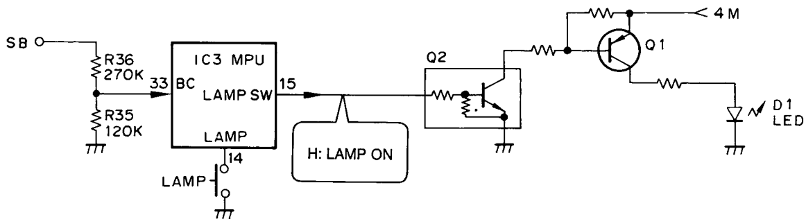
Fig. 13 Battery Voltage Detection Circuit and Lamp Circuit
